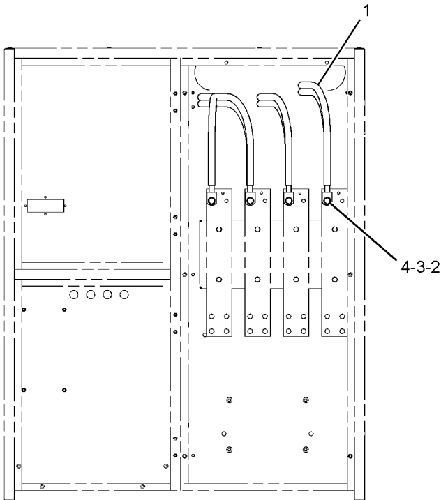
(BREAKER CONNECTION)
