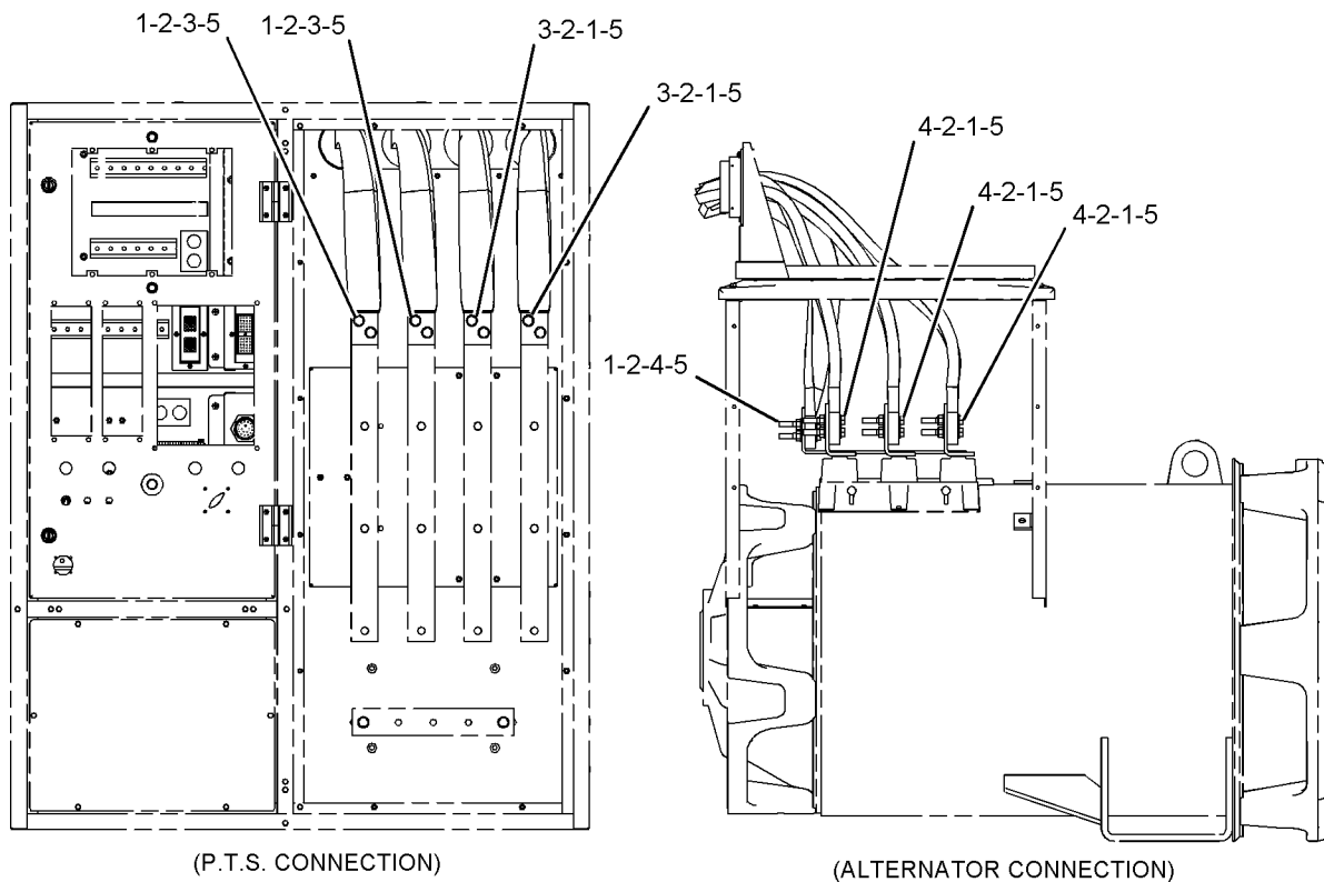
(ALTERNATOR CONNECTION)
