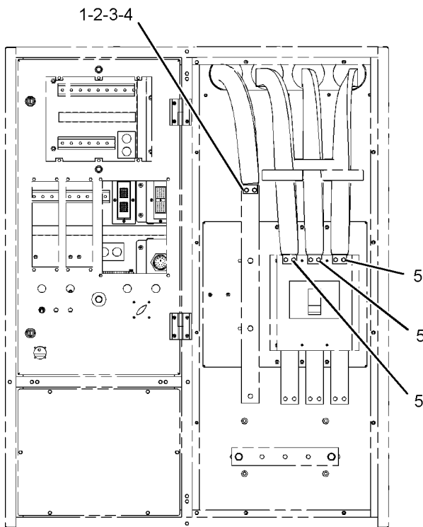
(BREAKER CONNECTION)
