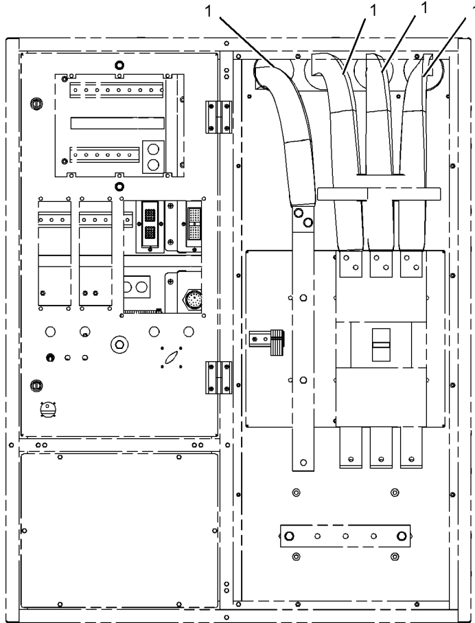
(BREAKER CONNECTION) <END>
