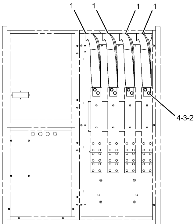
(BREAKER CONNECTION)
